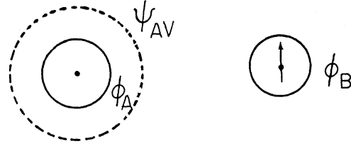
FIG. 2. Model system for nuclear moment centered on site B.
